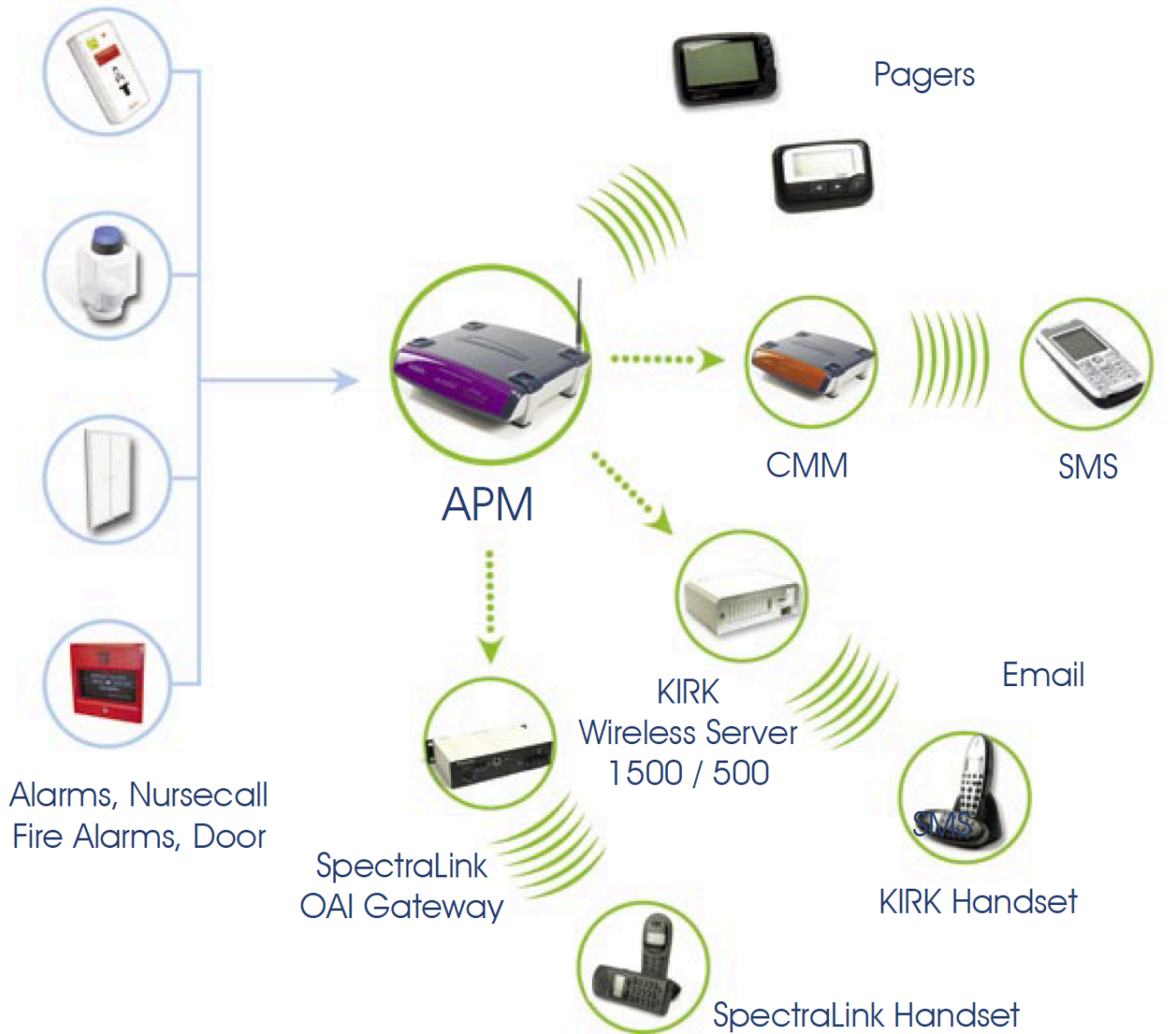
Typical System Schematic
